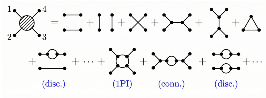
Figure 3.2: Diagrammatic expansion of the 4-point function for a cubic interaction up to second order in perturbation theory.
